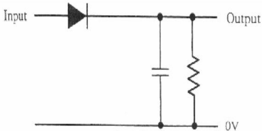
Figure 4: Diode Detector
