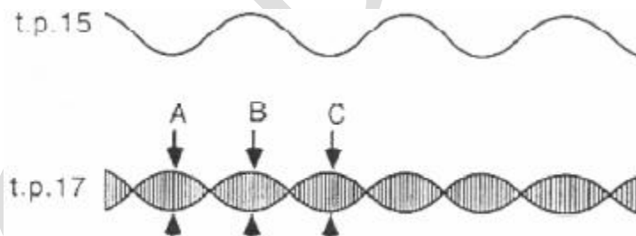
Figure 2: Modulating and Modulated Signal waveform
